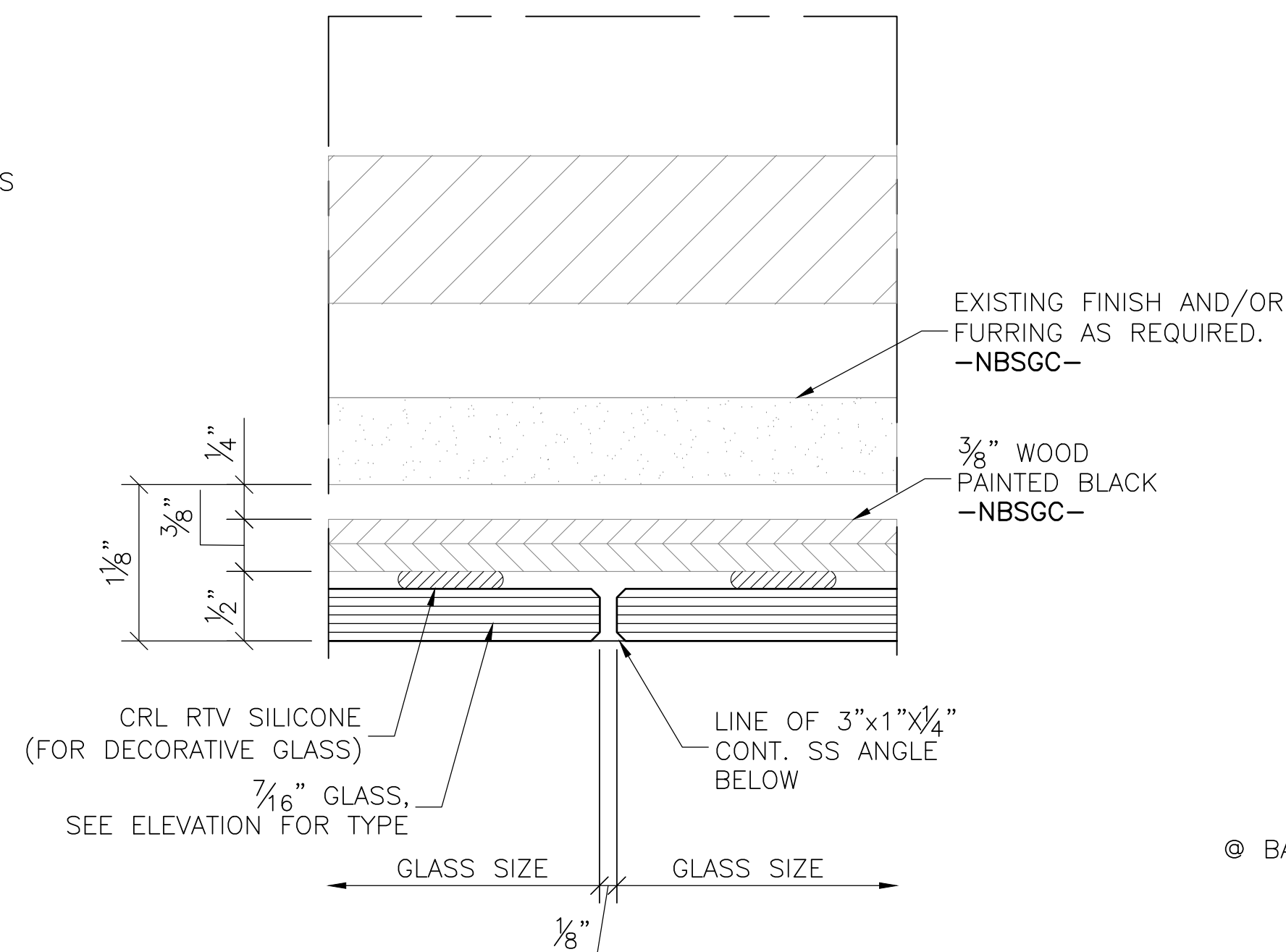
V2 ELEVATOR JAMB © BACK PAINTED GLASS ARCH REF: NONE
