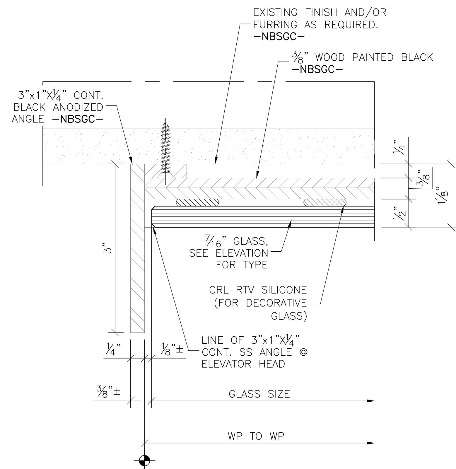
V1 OPEN JAMB © BACK PAINTED GLASS ARCH REF: NONE
