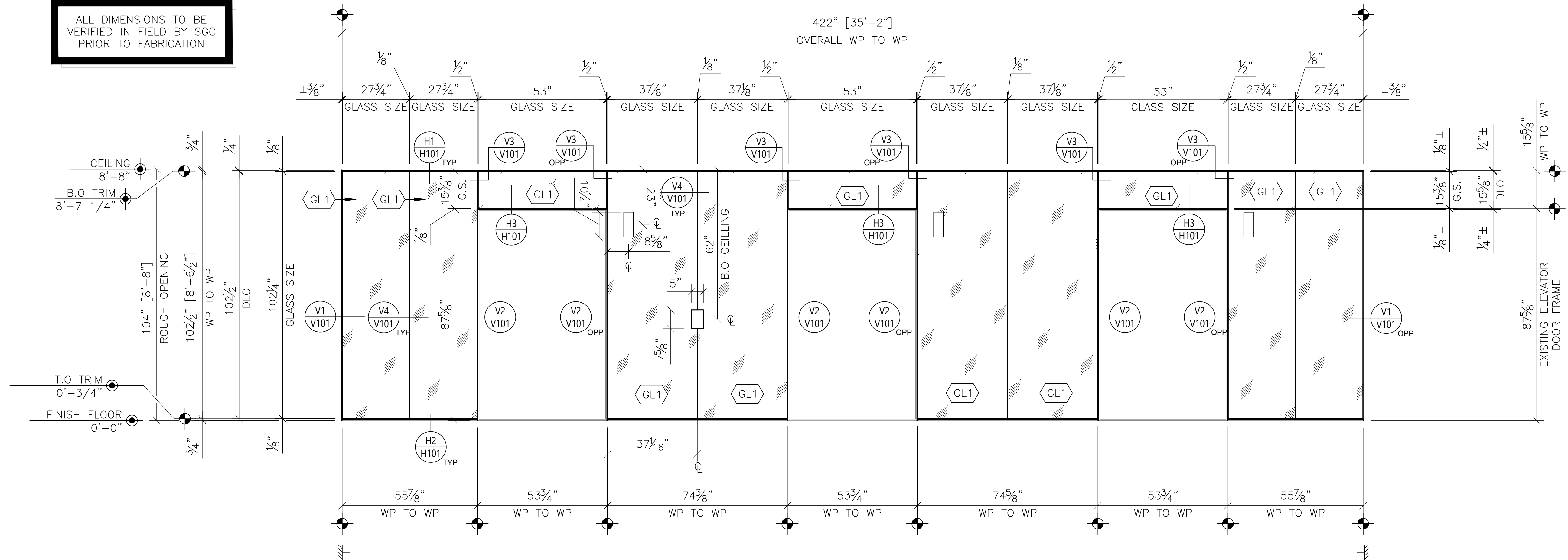
1 ELEVATION—EAST QUANTITY: 1 ARCH. REF: 4/A803 © ELEVATOR LOBBY 5100
