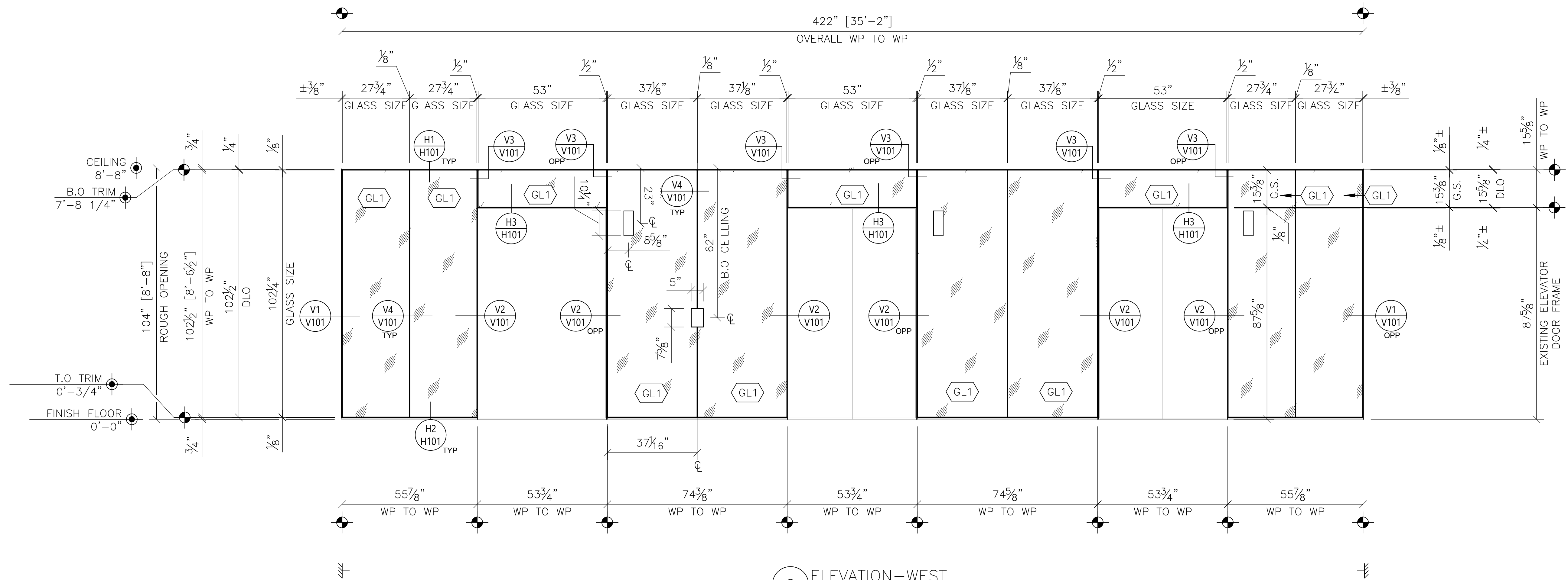
2 ELEVATION—WEST QUANTITY: 1 ARCH. REF: 2/A803 © ELEVATOR LOBBY 5100
