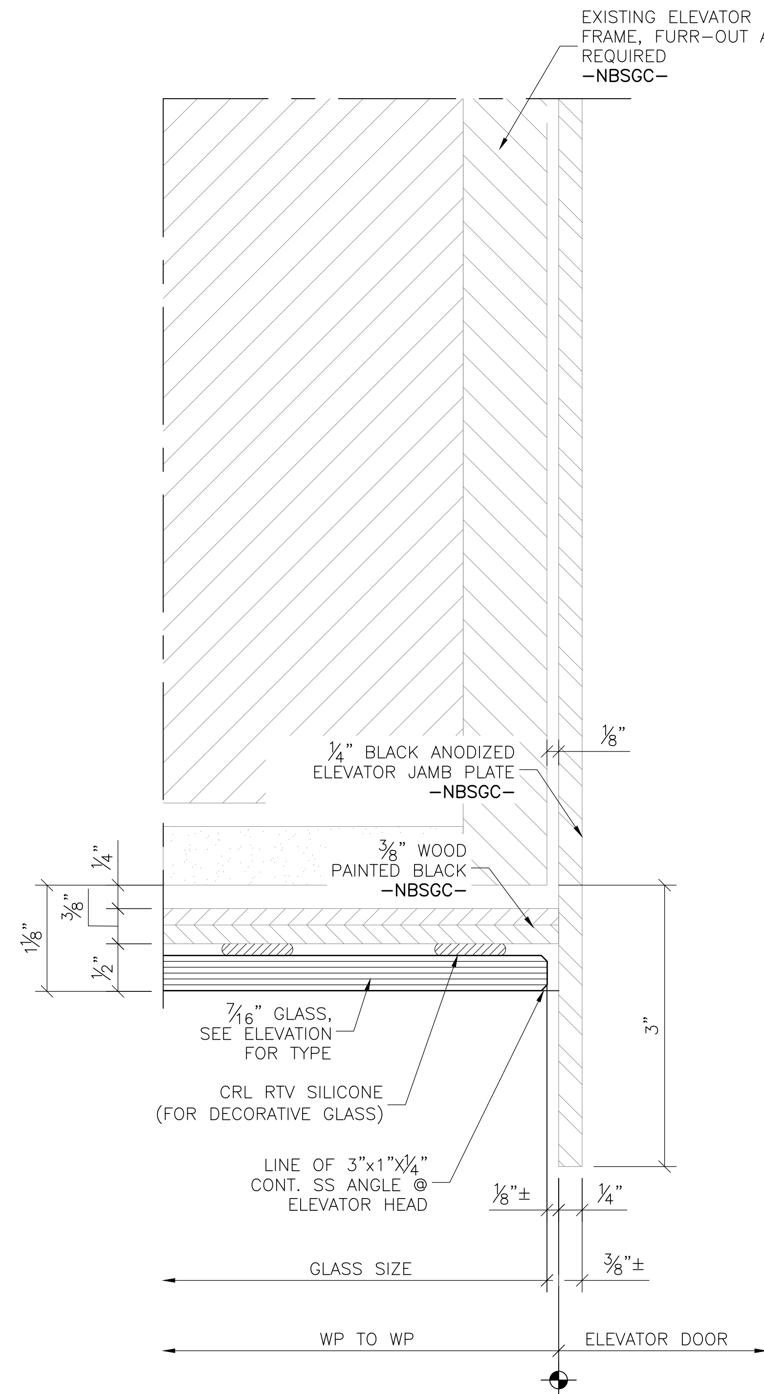
V2 ELEVATOR JAMB © BACK PAINTED GLASS ARCH REF: NONE
